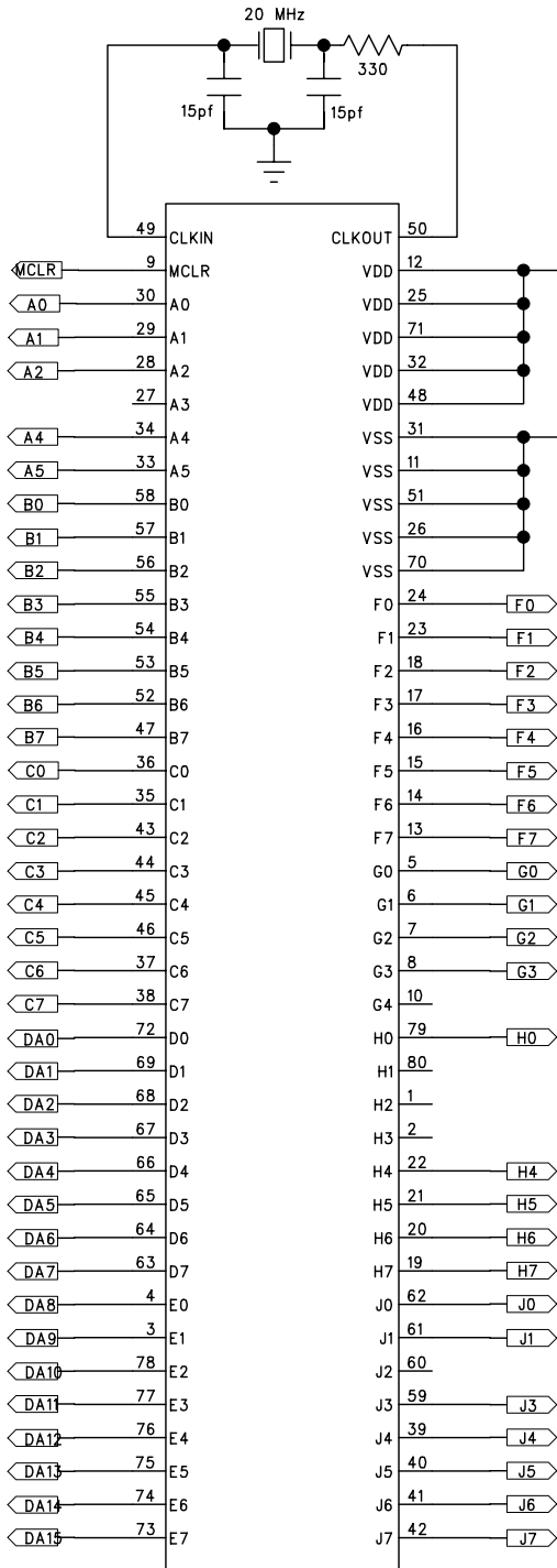
PIC18F8722
